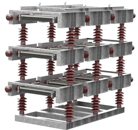
IP00 resistor: 3 x 38R 3 x 67kW Insulation Level: 36 kV.
