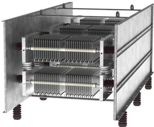
IP00 resistor: 3 x 7R 3 x 18kW Insulation Level: 12 kV.
